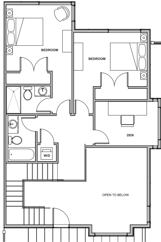
UPPER FLOOR
