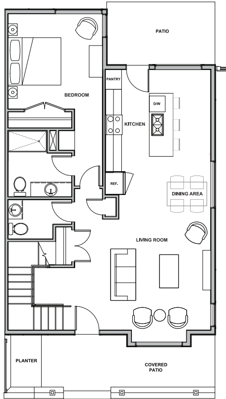
MAIN FLOOR
