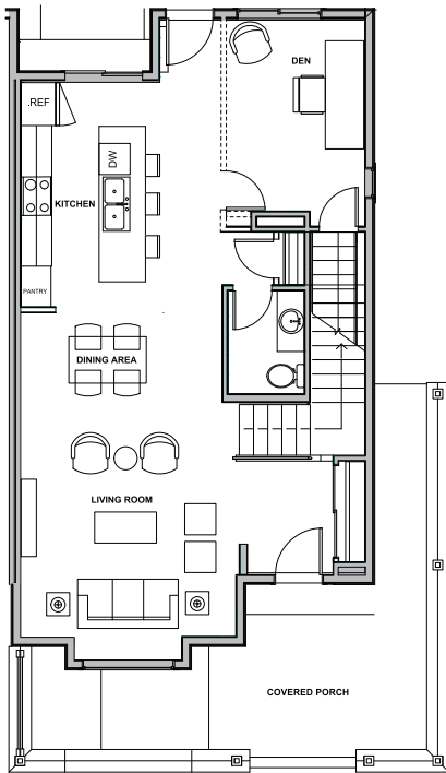
MAIN FLOOR
