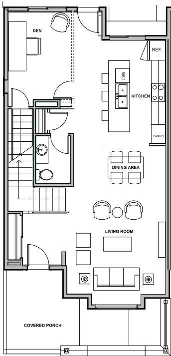
MAIN FLOOR
